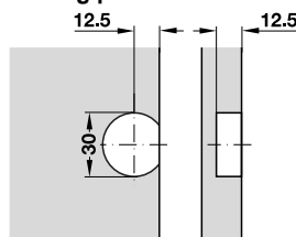
Detail view: Flap made of wood
